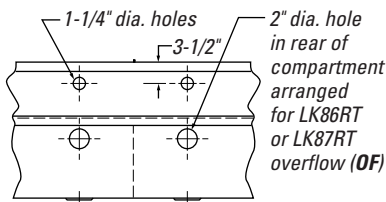
1-hole over each compartment and 2 overflow holes (OF) (MODEL NUMBER)OF _
