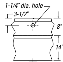
1-hole over compartment (MODEL NUMBER)1
