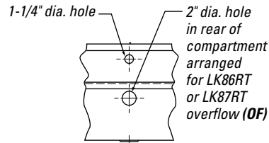
1-hole over compartment and 1 overflow hole (OF) (MODEL NUMBER)OF 1
