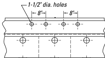
2-holes over partitions and 3 overflow holes (OF) (MODEL NUMBER)OF 4
