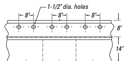
2-holes over each compartment (MODEL NUMBER)6
