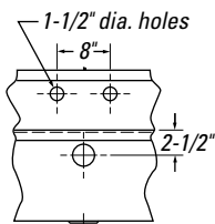
2-holes over compartment and 1 overflow hole (OF) (MODEL NUMBER)OF 2
